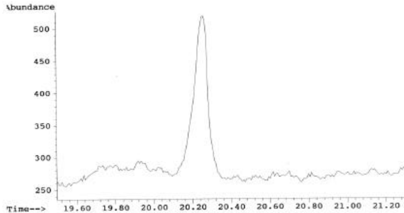
Figure 7: Pyrogram of wood treated with Thiabendazole 1.5 years prior to analysis. The minced wood samples were desorbed for 2 minutes at 290°C. The temperature program was 70°C-1 min-8°C/min-300°C-1min. The column used was a HP-5 (95%-methyl-5%-phenyl polysiloxane) 30 m x .25 µm x .25mm.
