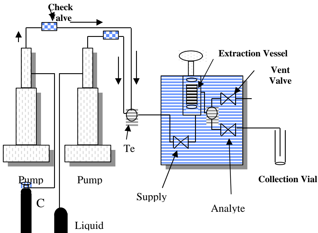
Figure 11: Schematic of Instrumental setup for ASE and SFE (37)
