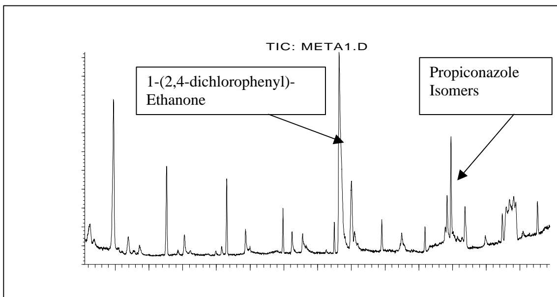
Figure 52: Total Ion Chromatogram of Degradation Products of Propiconazole
