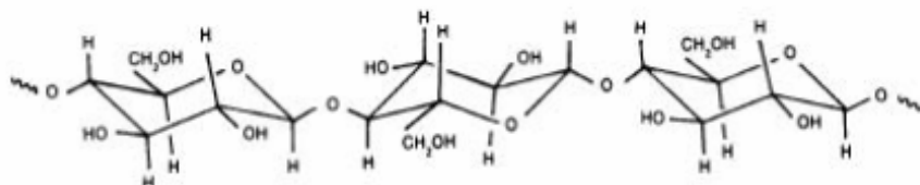
Figure 37: Structure of Cellulose
