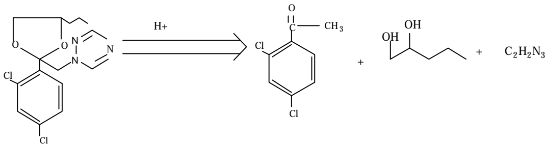
Figure 54: Experimental Degradation Pathway (84)
