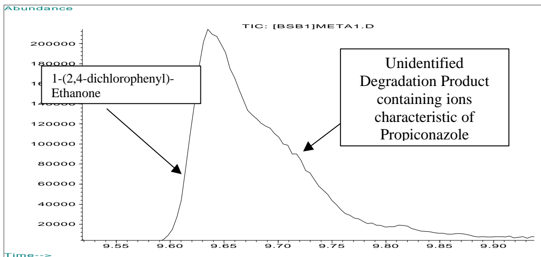
Figure 57: Enlarged Total Ion Chromatogram (TIC) of Degradation Product
