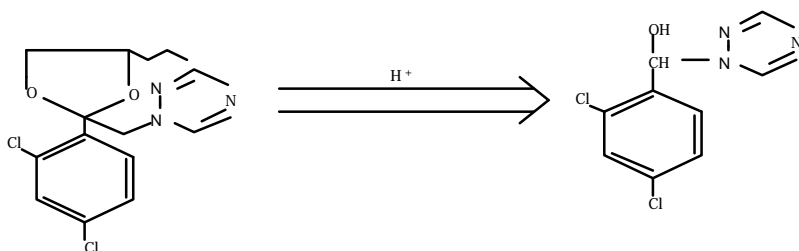
Figure 47: Proposed Degradation Pathway of Propiconazole
