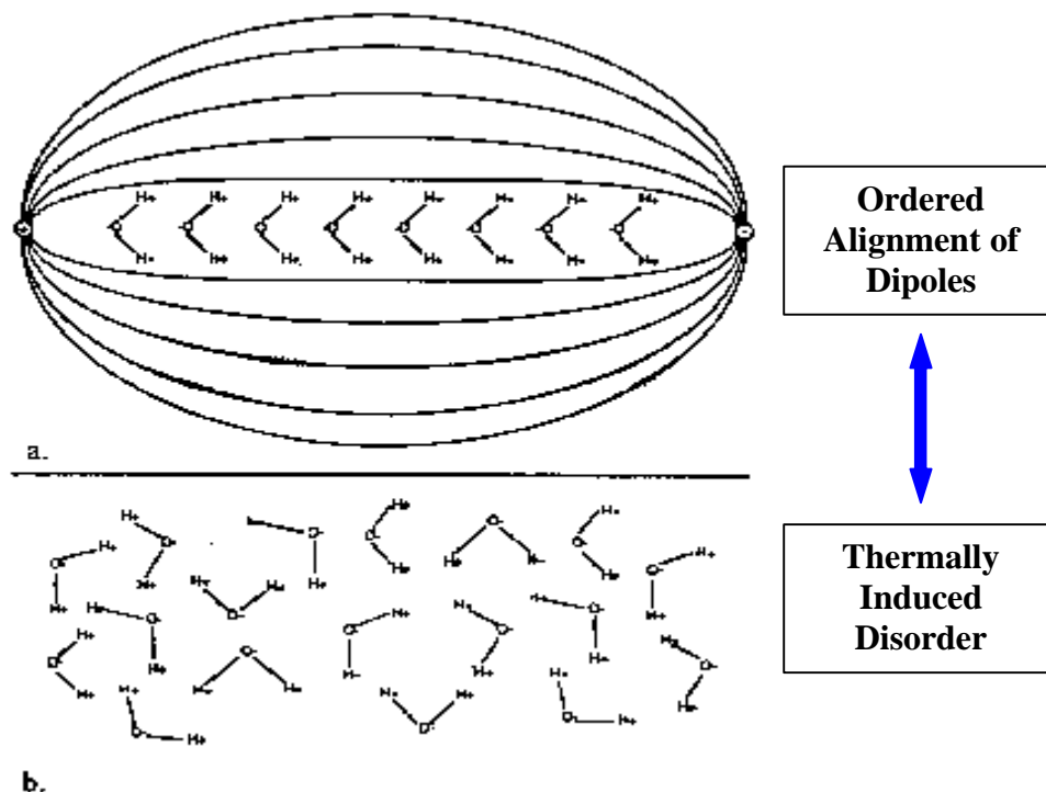
Figure 12: Effects of Microwaves on Water (46)
