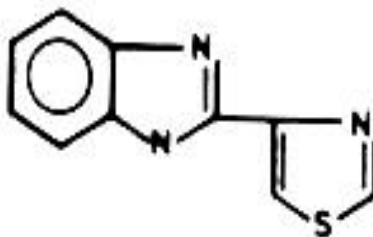
Figure 6: Chemical Structure of Thiabendazole
