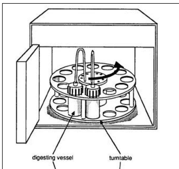
Figure 13: Schematic of a Closed-Vessel System (46)
