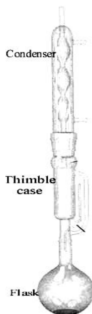
Figure 9: Schematic of Soxhlet Extraction Apparatus (19)
